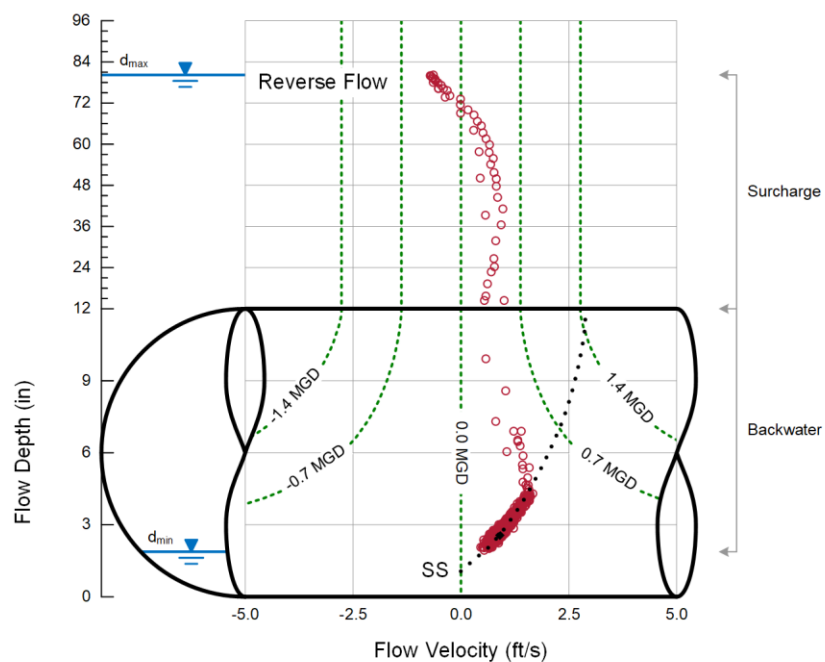
FIGURE 10: Scattergraph of Reverse Flow
