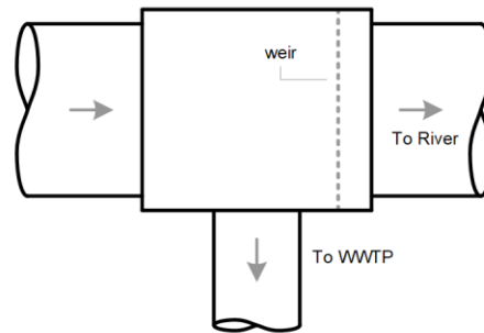
FIGURE 11: Plan View of a CSO Regulator with an End Weir
