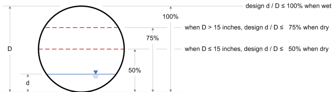
FIGURE 1: Flow Depth-to-Diameter Ratio in the Context of Sewer Design Criteria
