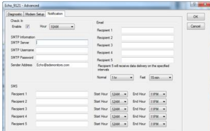
Notification Tab of Advanced Device Dialog
